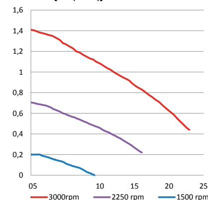
Curva H/Q [Bar(m³/h)]
